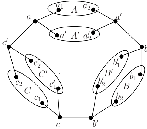
Figure 2: Labeling of the graph G
