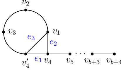
Figure 3.5: H_b - \{v_3 v_4\} .
